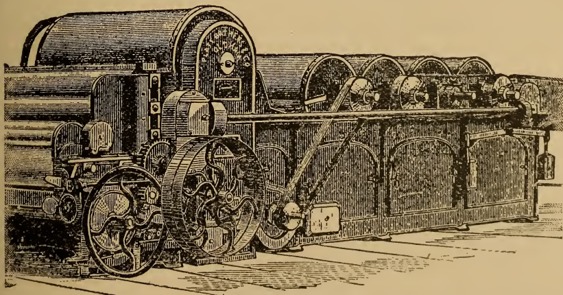
Fig. 142. THREE-CYLINDER COTTON OPENER, BEATER AND LAP MACHINE.
